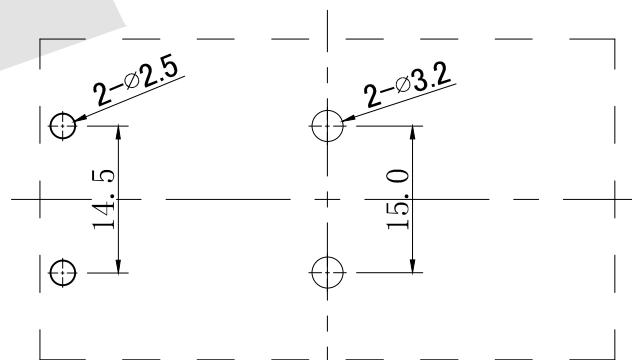
MOUNTING DETAIL
