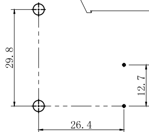
MOUNTING DETAIL
